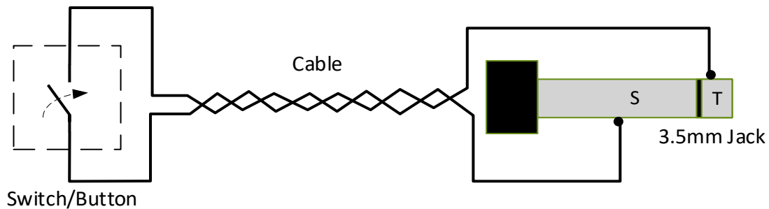
Figure 5 DIGITAL INPUT PASSIVE SWITCH
