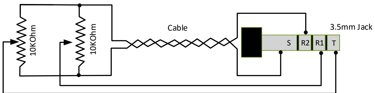
Figure 7 PASSIVE JOYSTICK DEVICE
